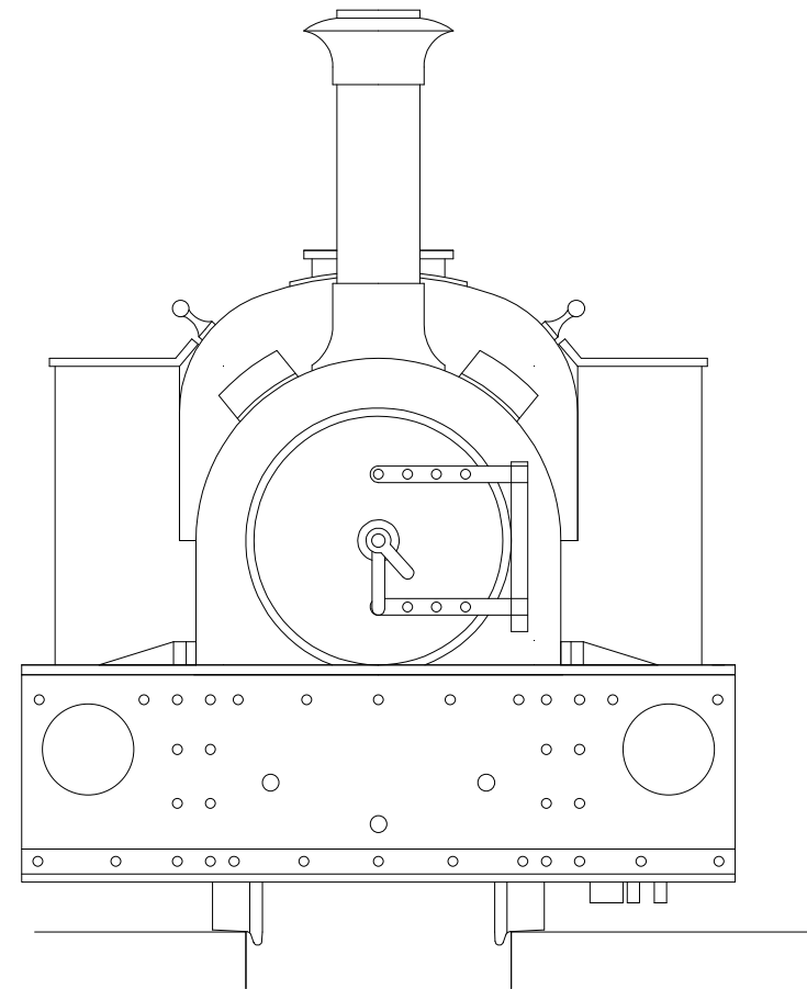
Wild Rose III sheet 2 General Arrangement - End Elevation
