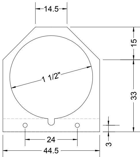
Front boiler support. Dotted line shows position of frame spacer Bolt to frame spacer
