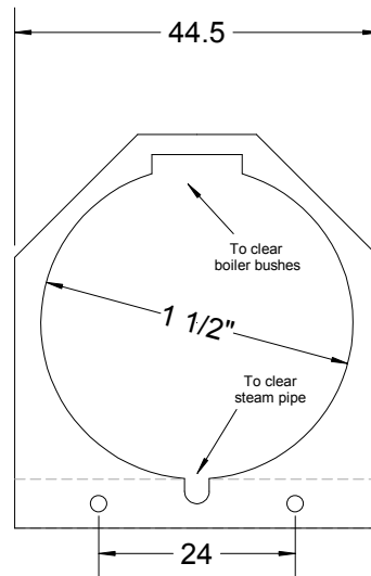
Rear boiler support Dotted line shows position of frame spacer Bolt to frame spacer
