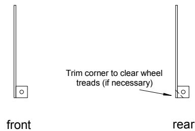
Assembled boiler supports and frame spacers, half full size
